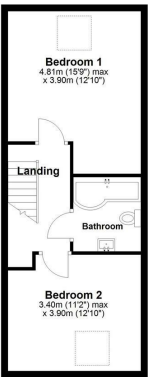
First Floor Approx. 40.9 sq. metres (440.8 sq. feet)
